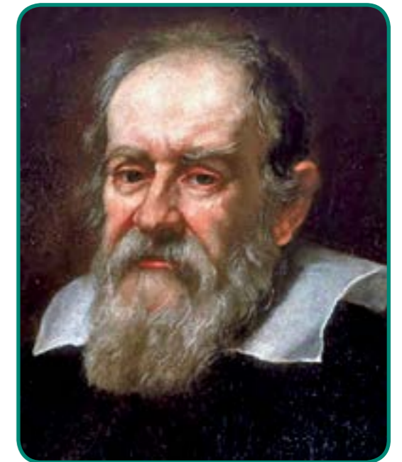
Galileo Galilei
